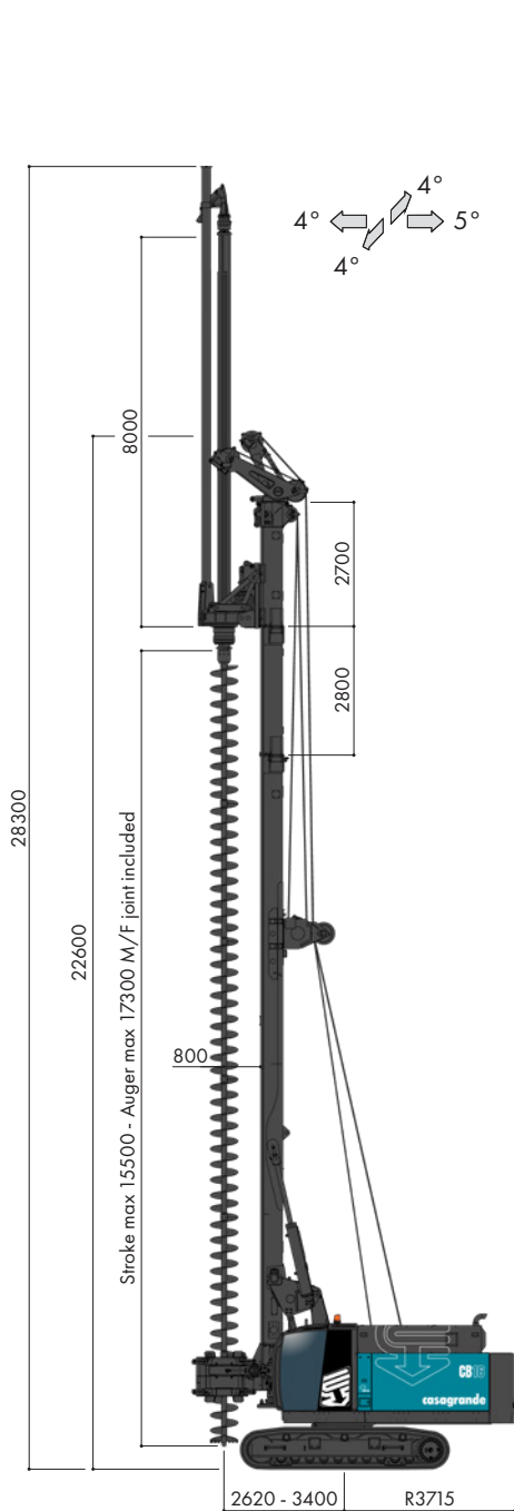
CFA-R ARRANGEMENT
