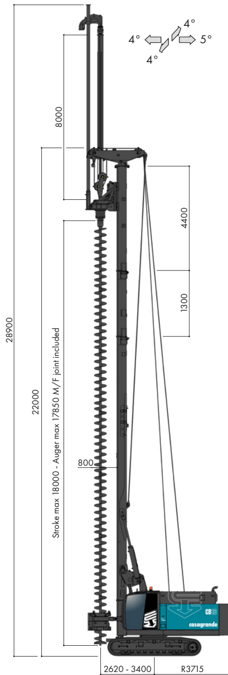
CFA ARRANGEMENT
