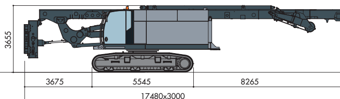
Base carrier with mast without counterweight Carro base con mast senza zavorra ~ 61200 kg
